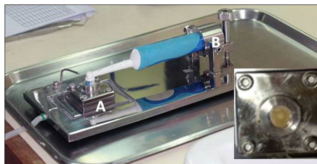
Figure 1: Tooth brushing device (A) a dentine disk holder and (B) a toothbrush holder. The inset shows a top-down view
